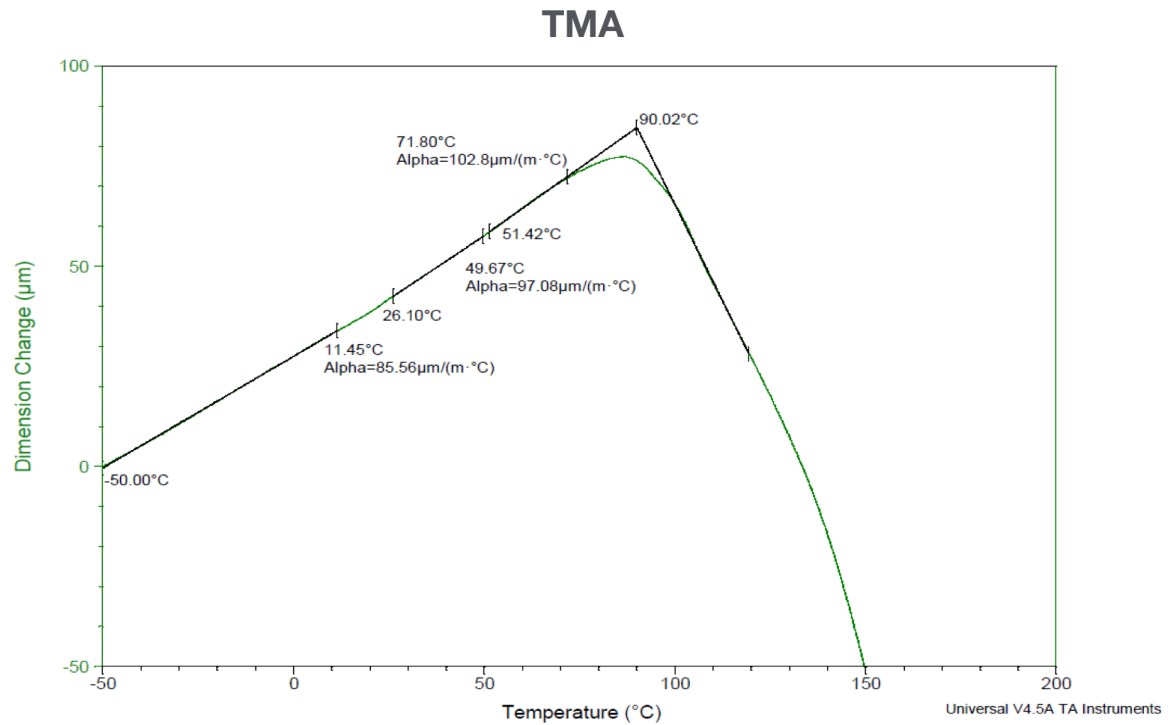
Figure 3. Dimension change data as a function of temperature for the Nylon 12 On Edge (XZ) sample.
